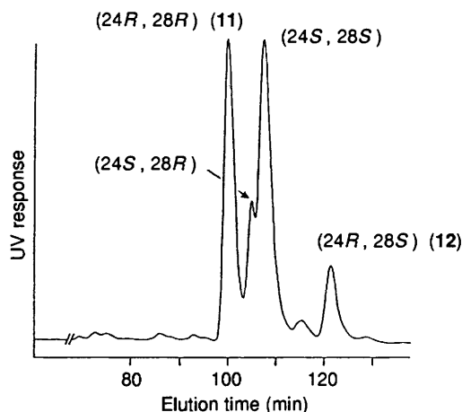
Figure 1. HPLC separation of the diastereoisomeric mixture of epoxide benzoates. Conditions: column, a Shim-pack CLC SIL ( 15 \times 0.6 cm i.d.); eluting solvent hexane-dichloromethane (2:1); flow rate 2 ml \text{min}^{-1} ; detected with a UV monitor at 230 nm. It was previously known that the (24 R ,28 R )-epoxide is more mobile than the (24 S ,28 S )-isomer (Y. Fujimoto and N. Ikekawa, J. Org. Chem. , 1980, 45, 566; N. Ikekawa, Y. Fujimoto, A. Takasu, and M. Morisaki, J. Chem. Soc., Chem. Commun. , 1980, 709). The elution order of isofucoesterol (24 R ,28 S )- and (24 R ,28 S )-epoxide benzoates was determined in the present work by conversion of the stereochemically defined isomeric acetates (ref. 14) into the corresponding benzoates.
